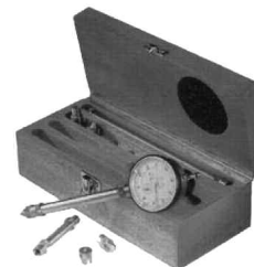
Crankshaft Deflection Gauge (60-580 mm)
