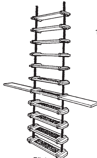
Pilot Ladder 11
